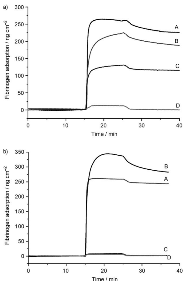
Figure 5. a) Representative SPR sensorgrams showing the adsorption of fibrinogen ( 1 \text{ mg mL}^{-1} ) in PBS buffer on the surfaces grafted with pCBMA-1 C2 by ATRP A) before hydrolysis and after hydrolysis for 24 h with B) H 2 O, C) CEHS (10 mM, pH 9.0), and D) CAPS (10 mM, pH 10.0). b) Representative SPR sensorgrams showing the adsorption of 1 \text{ mg mL}^{-1} fibrinogen in PBS buffer on the surfaces grafted with pC8NMA A) before and B) after incubation for 24 h with CAPS (10 mM, pH 10.0), and on surfaces grafted with pCBMA-2 C) before hydrolysis and D) after hydrolysis for 24 h with CAPS (10 mM, pH 10.0).
